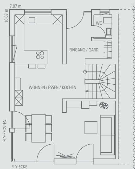
Erdgeschoss, ca. 58 m 2 NGF.
